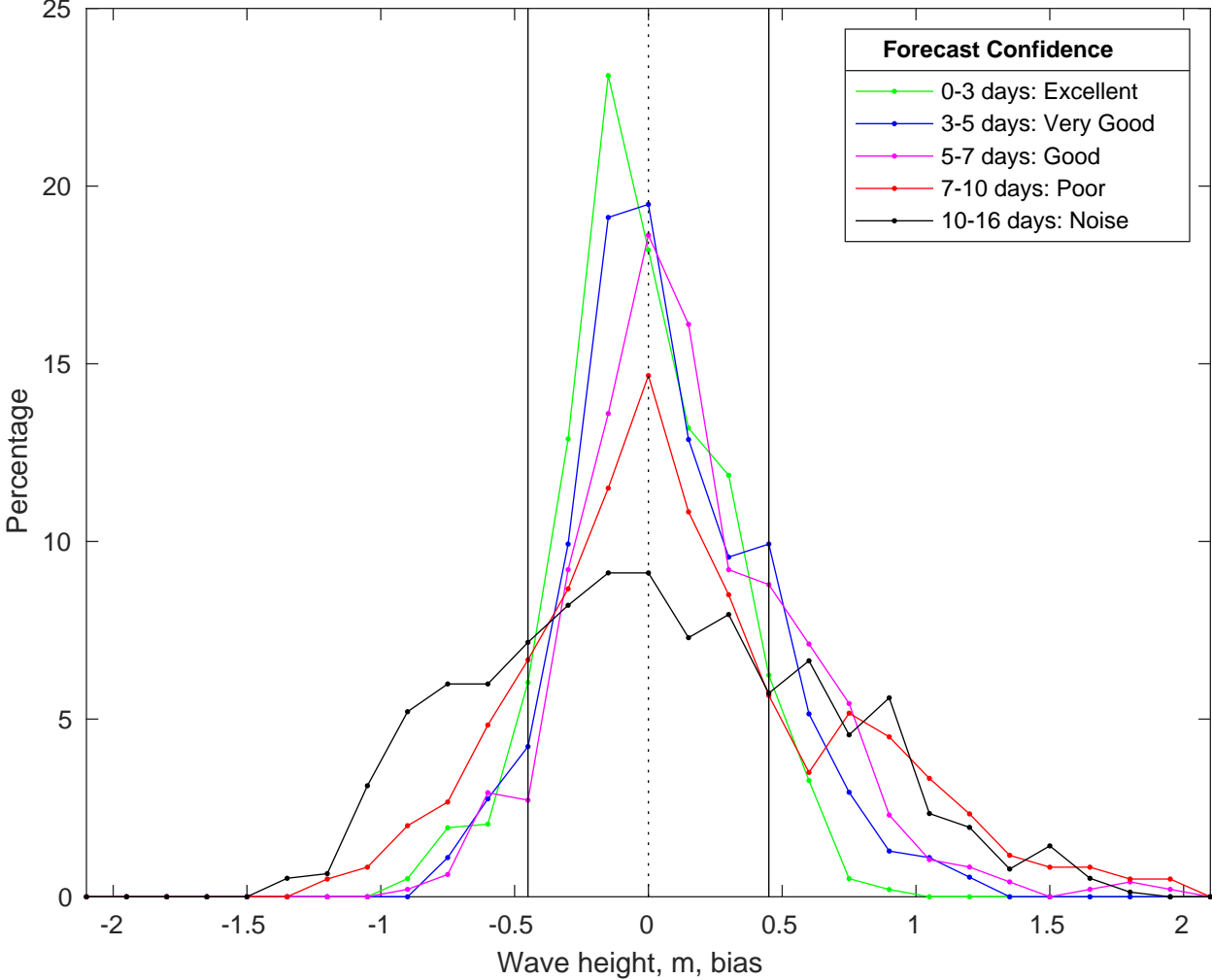
NDBC 46028 vs GFS Waves Bias Histogram: 13-Jul-2025
