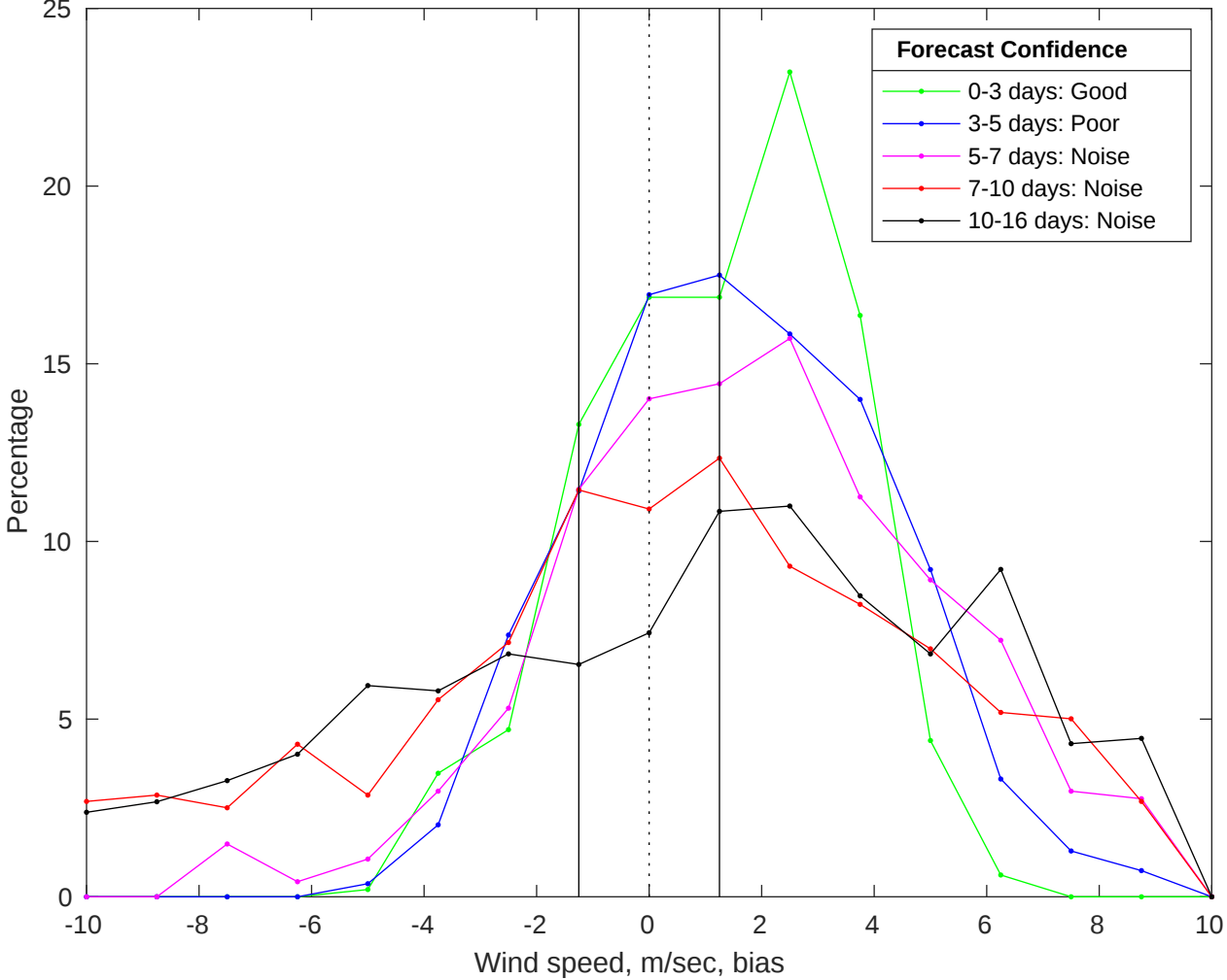
NDBC 46028 vs GFS Winds Bias Histogram: 13-Jul-2025
