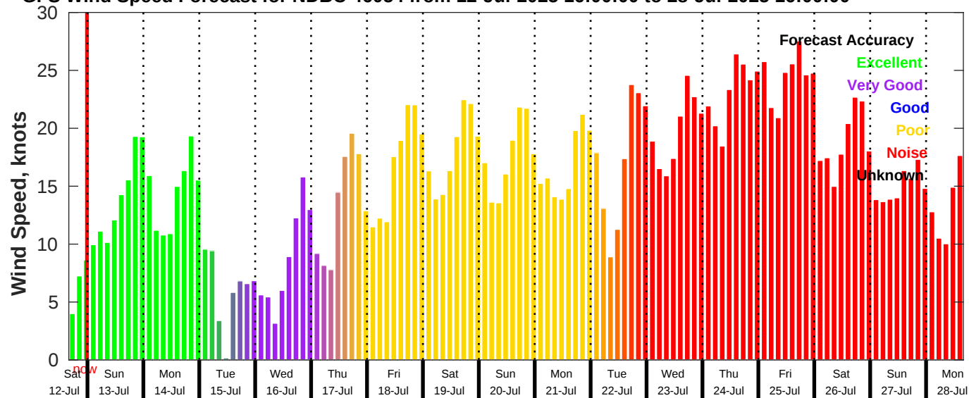
GFS Wind Speed Forecast for NDBC 46054 from 12-Jul-2025 16:00:00 to 28-Jul-2025 16:00:00
