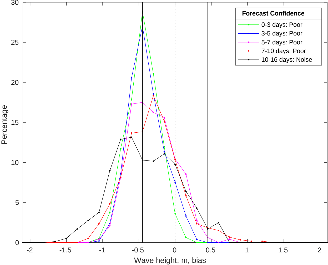
NDBC 46069 vs GFS Waves Bias Histogram: 13-Jul-2025
