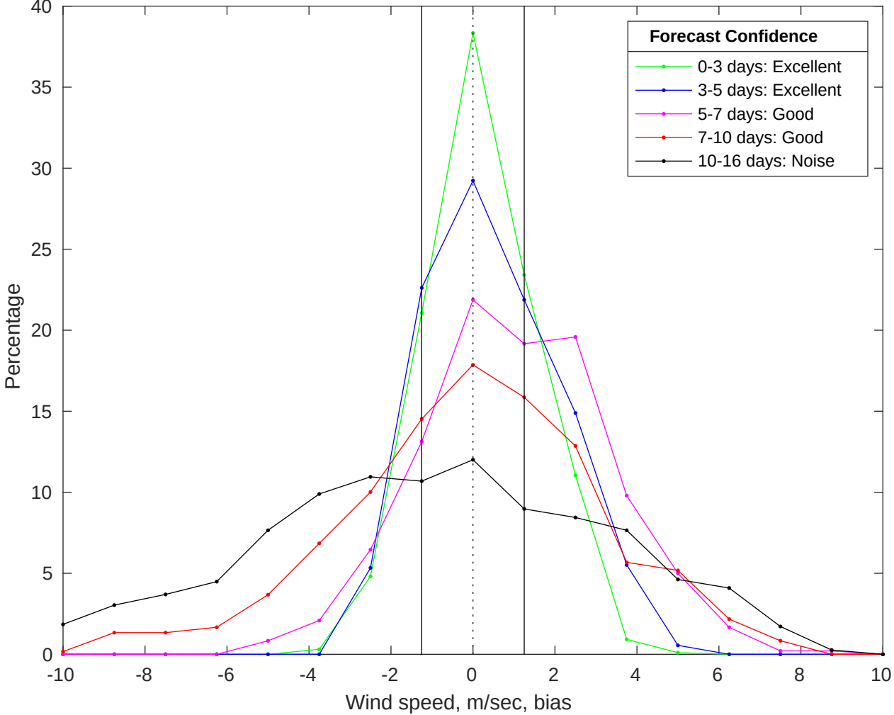
NDBC 46069 vs GFS Winds Bias Histogram: 13-Jul-2025
