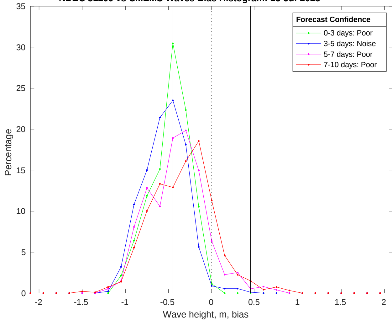
NDBC 51209 vs CMEMS Waves Bias Histogram: 13-Jul-2025
