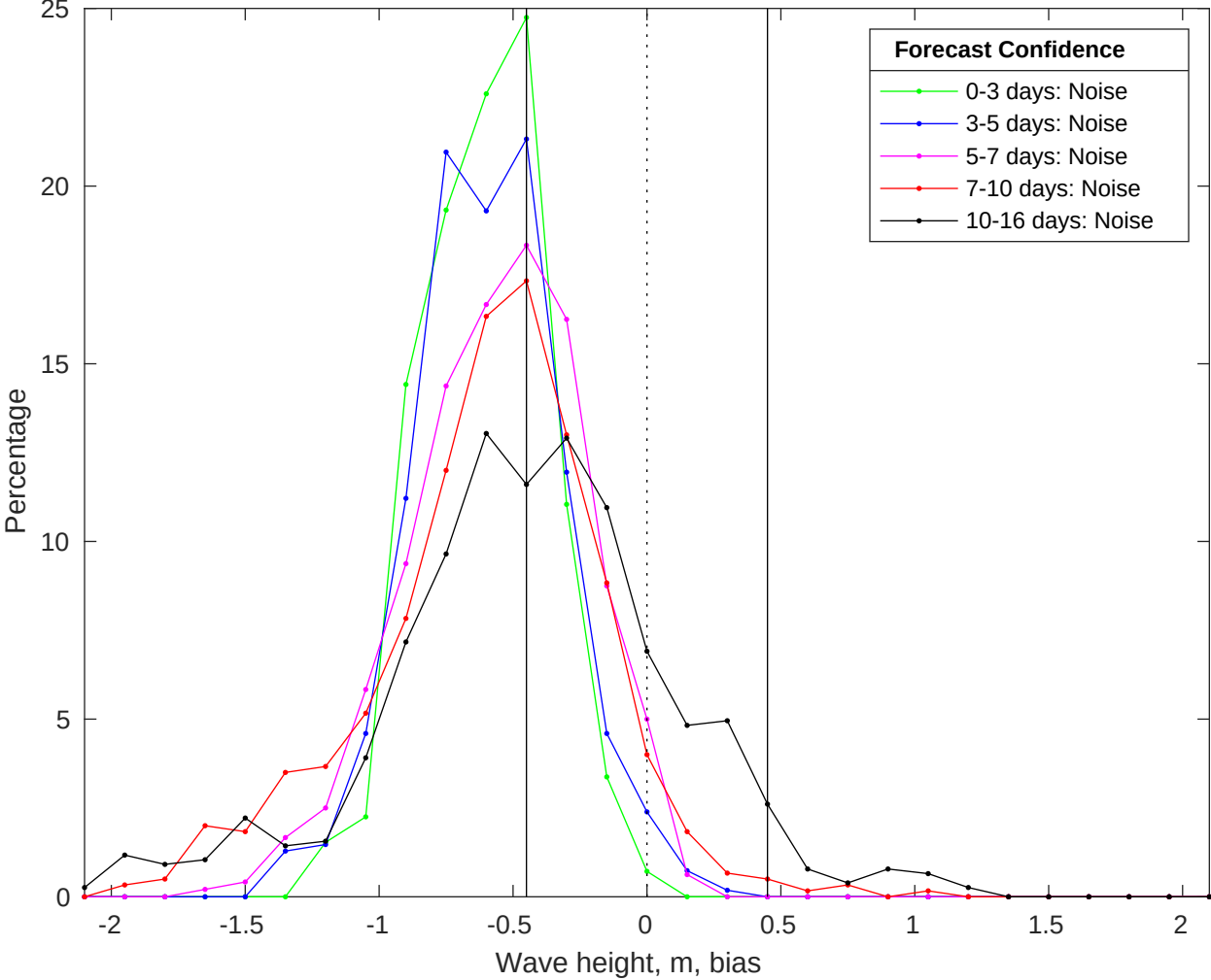
NDBC 51209 vs GFS Waves Bias Histogram: 13-Jul-2025
