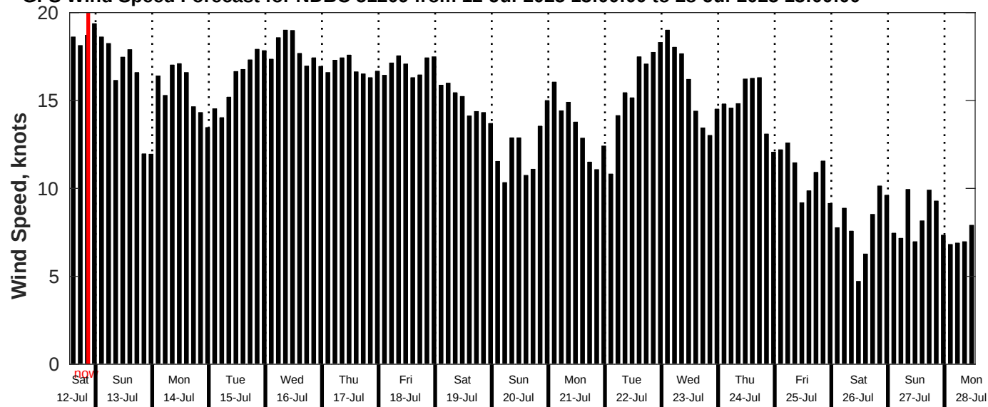
GFS Wind Speed Forecast for NDBC 51209 from 12-Jul-2025 13:00:00 to 28-Jul-2025 13:00:00
