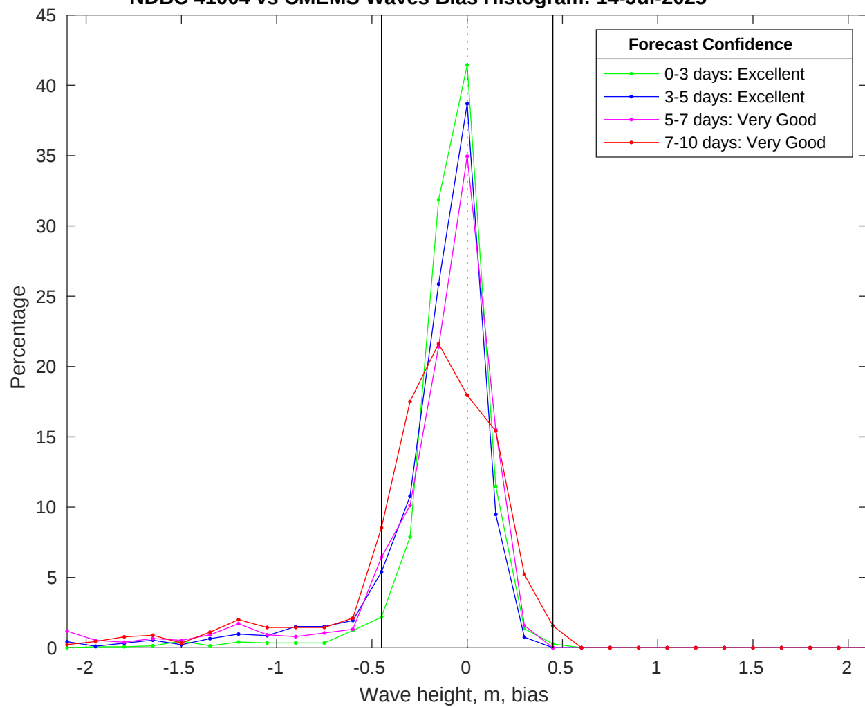
NDBC 41004 vs CMEMS Waves Bias Histogram: 14-Jul-2025
