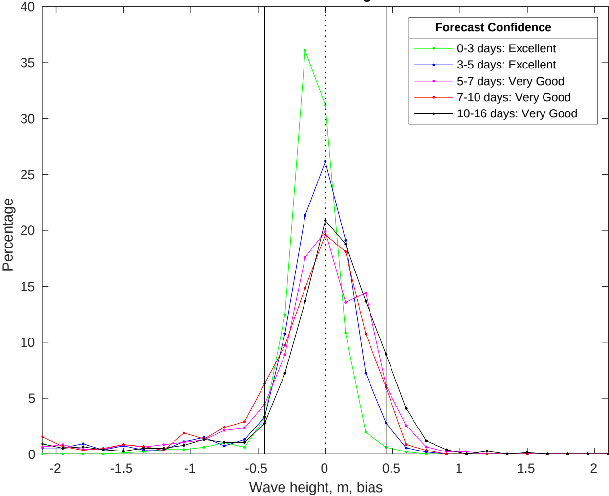
NDBC 41004 vs GFS Waves Bias Histogram: 14-Jul-2025
