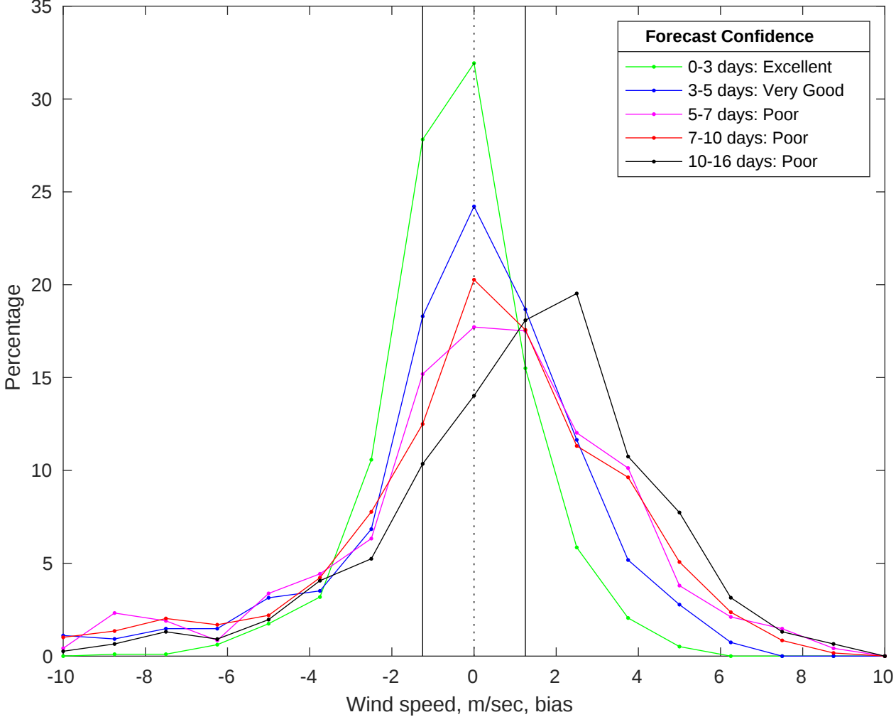
NDBC 41004 vs GFS Winds Bias Histogram: 14-Jul-2025
