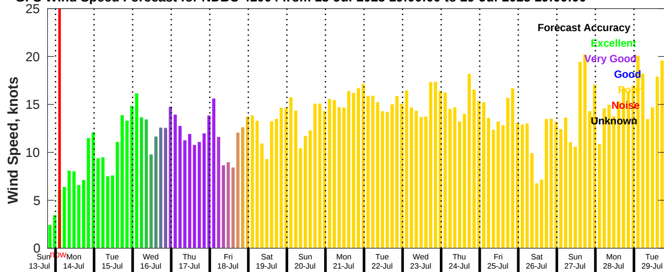
GFS Wind Speed Forecast for NDBC 41004 from 13-Jul-2025 19:00:00 to 29-Jul-2025 19:00:00
