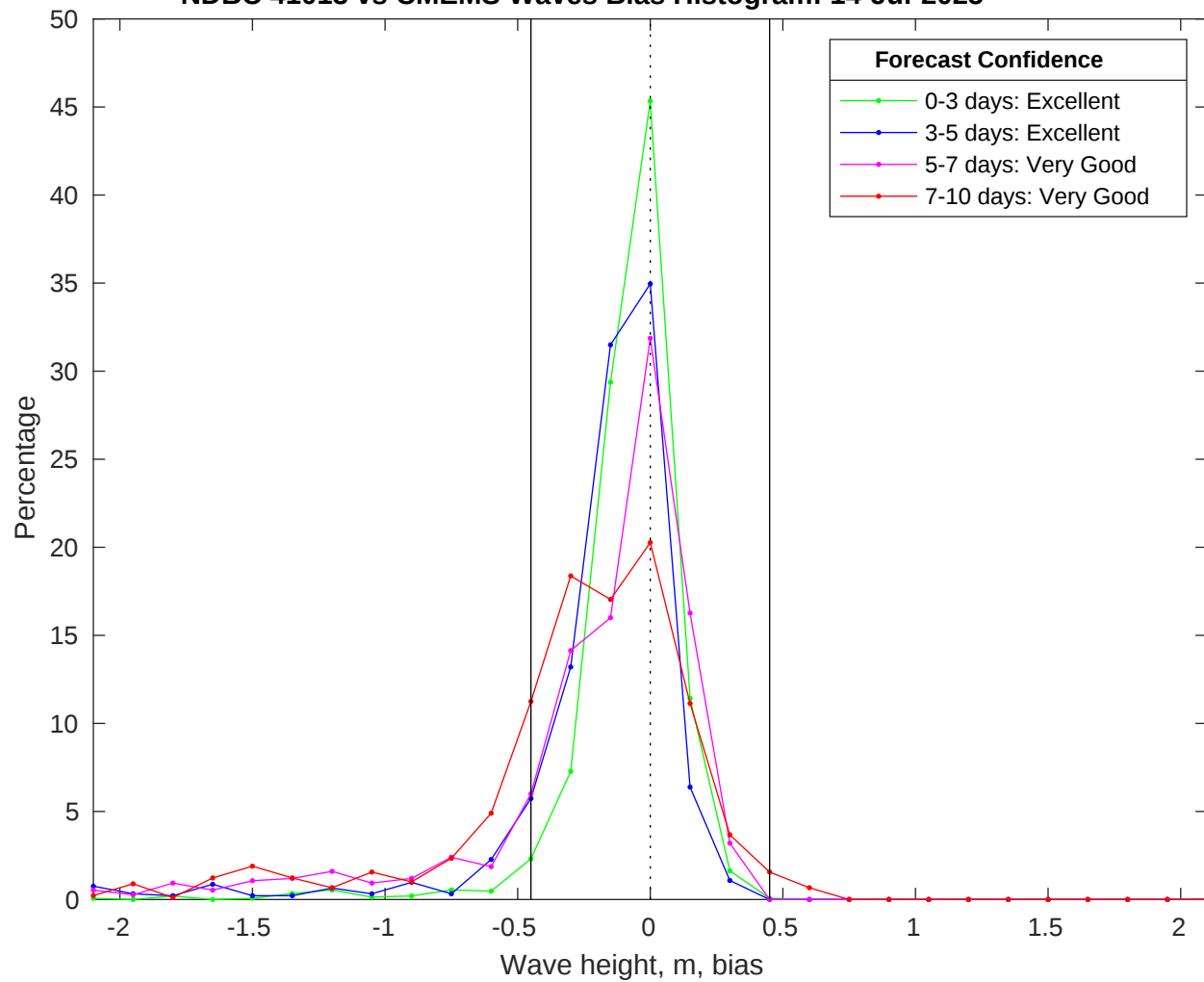
NDBC 41013 vs CMEMS Waves Bias Histogram: 14-Jul-2025
