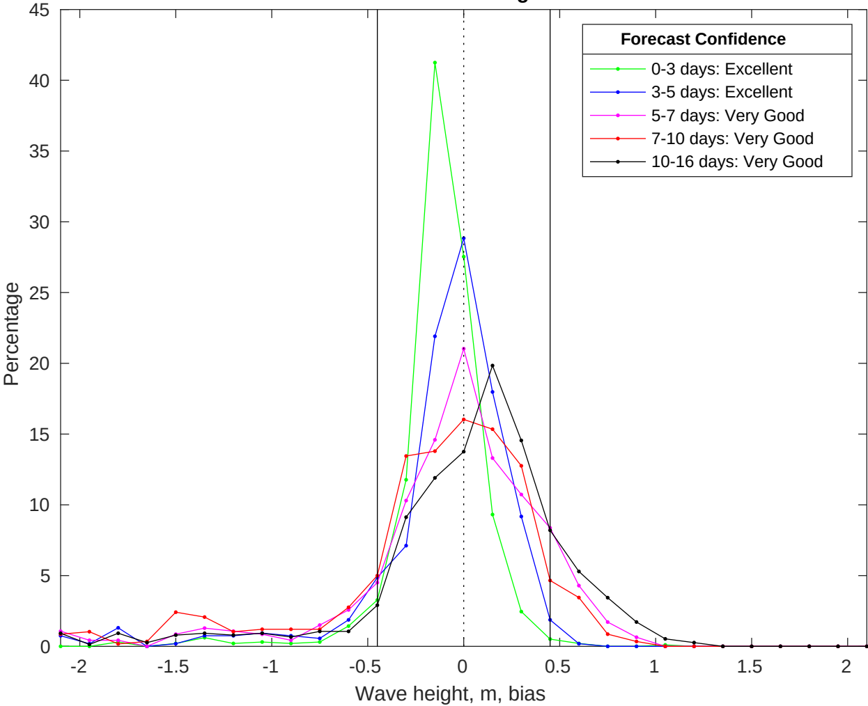
NDBC 41013 vs GFS Waves Bias Histogram: 14-Jul-2025
