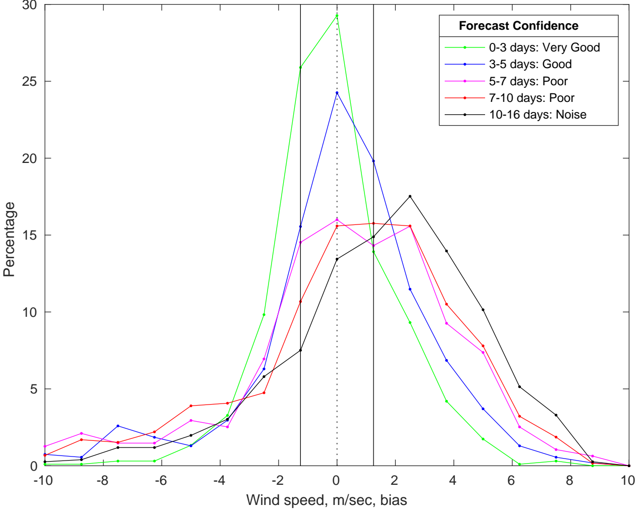
NDBC 41013 vs GFS Winds Bias Histogram: 14-Jul-2025
