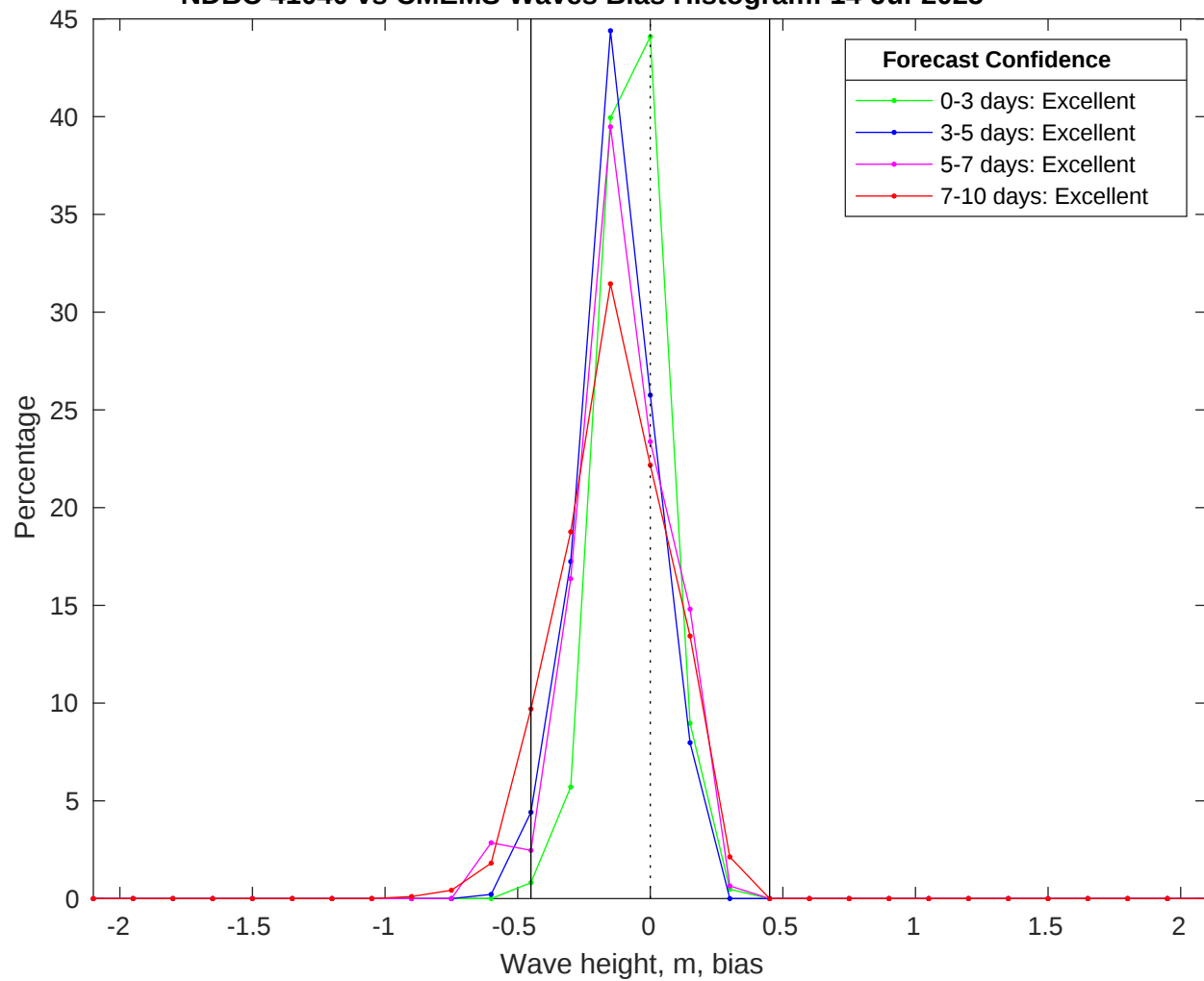
NDBC 41040 vs CMEMS Waves Bias Histogram: 14-Jul-2025
