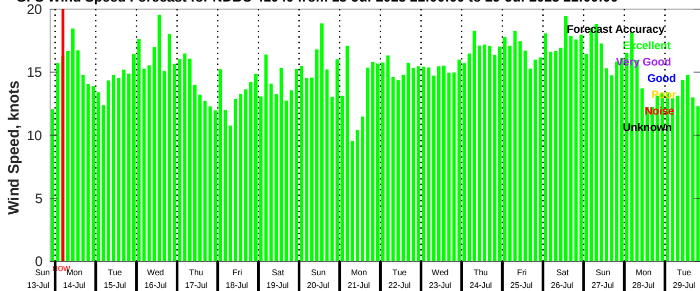
GFS Wind Speed Forecast for NDBC 41040 from 13-Jul-2025 21:00:00 to 29-Jul-2025 21:00:00
