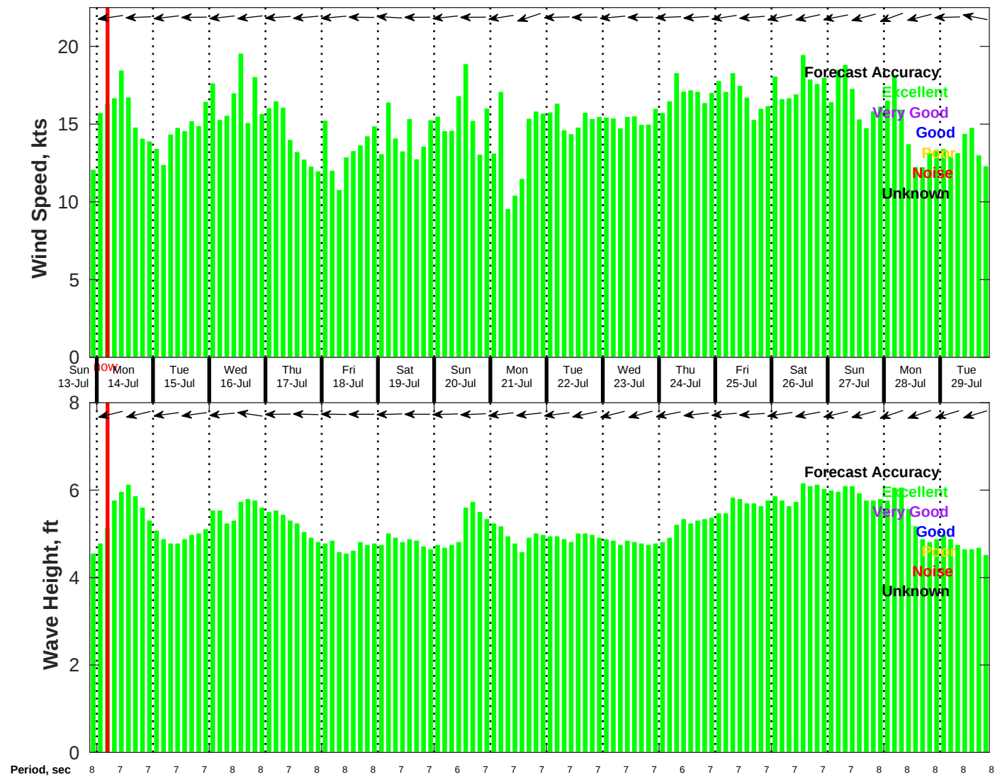
Wind & Wave Forecast for NDBC 41040 from 13-Jul-2025 21:00:00 to 29-Jul-2025 21:00:00
