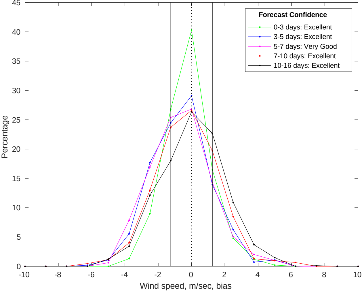
NDBC 42019 vs GFS Winds Bias Histogram: 14-Jul-2025
