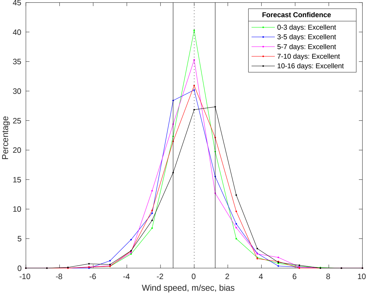
NDBC 42020 vs GFS Winds Bias Histogram: 14-Jul-2025
