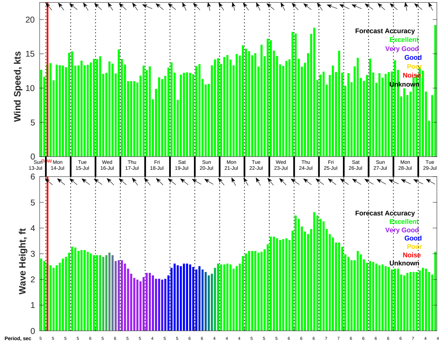
Wind & Wave Forecast for NDBC 42020 from 13-Jul-2025 18:00:00 to 29-Jul-2025 18:00:00
