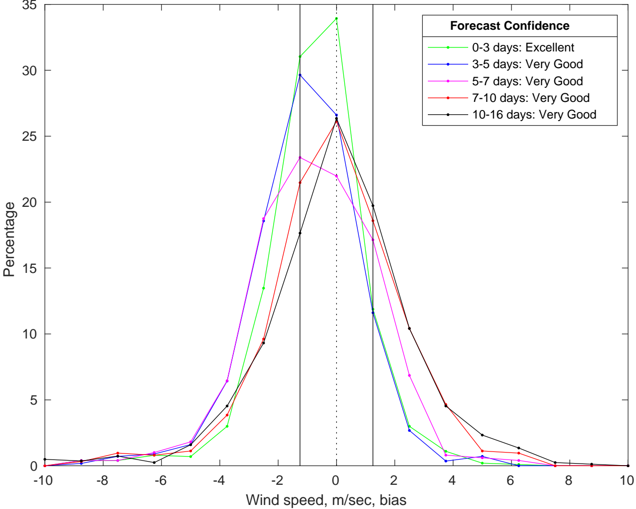
NDBC 42035 vs GFS Winds Bias Histogram: 14-Jul-2025
