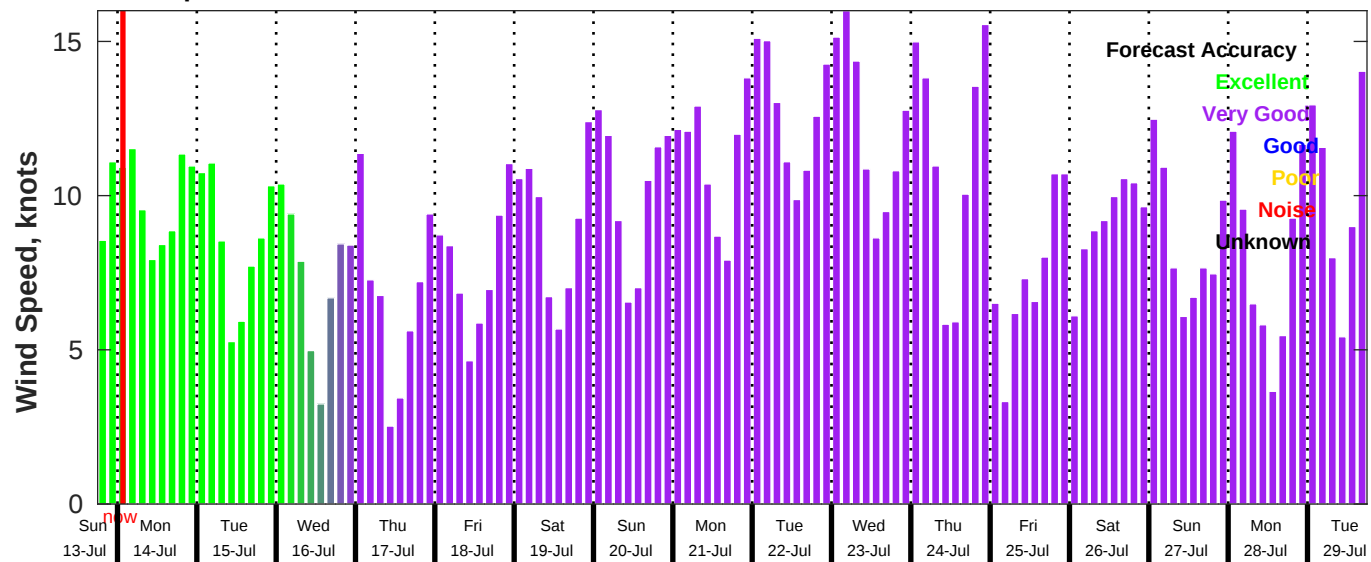
GFS Wind Speed Forecast for NDBC 42035 from 13-Jul-2025 18:00:00 to 29-Jul-2025 18:00:00
