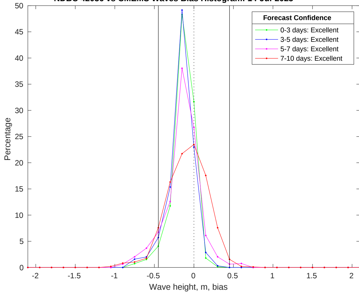
NDBC 42036 vs CMEMS Waves Bias Histogram: 14-Jul-2025
