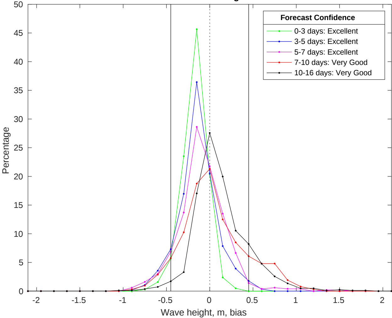
NDBC 42036 vs GFS Waves Bias Histogram: 14-Jul-2025
