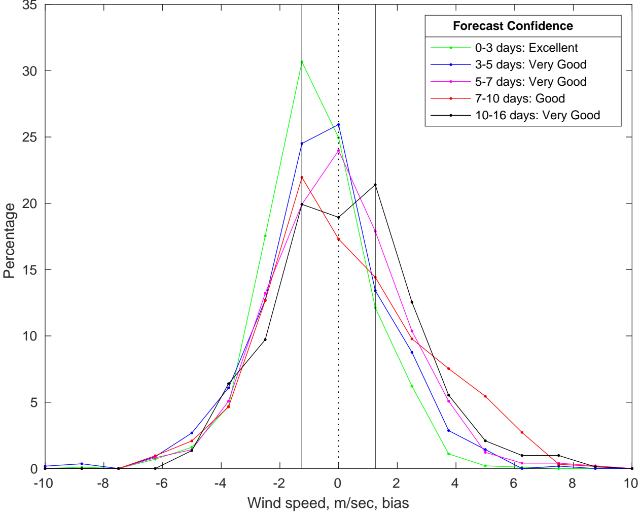
NDBC 42036 vs GFS Winds Bias Histogram: 14-Jul-2025
