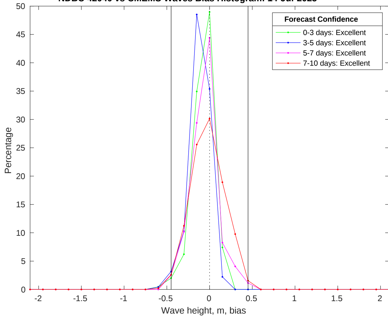
NDBC 42040 vs CMEMS Waves Bias Histogram: 14-Jul-2025
