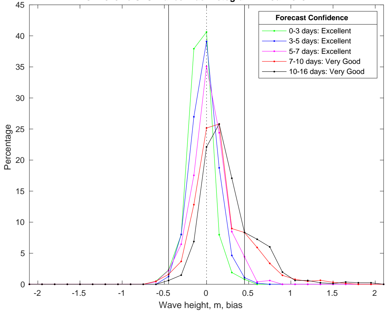
NDBC 42040 vs GFS Waves Bias Histogram: 14-Jul-2025
