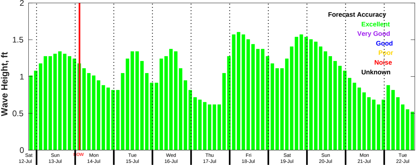
CMEMS Wave Forecast for NDBC 42040 from 12-Jul-2025 19:00:00 to 22-Jul-2025 19:00:00
