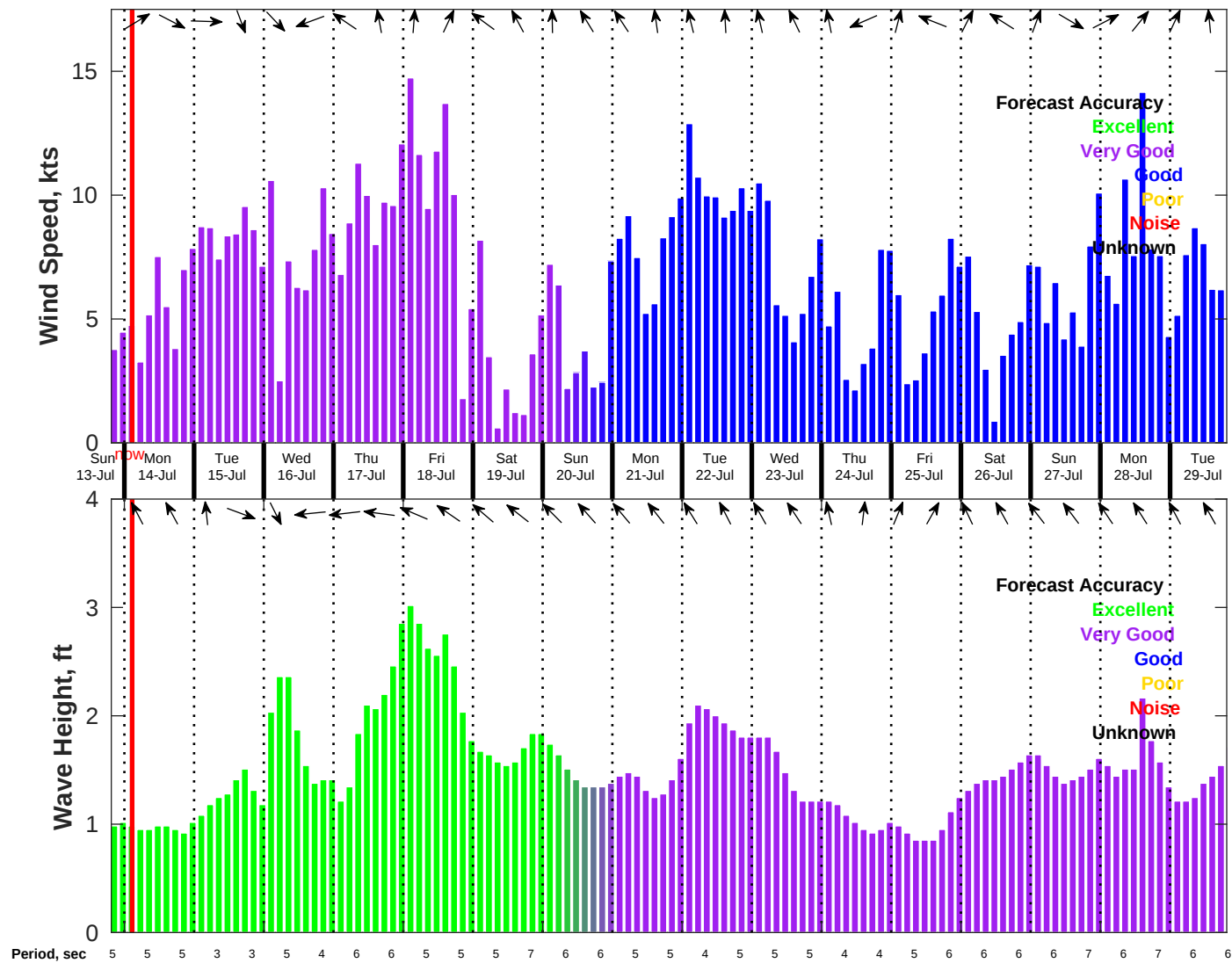
Wind & Wave Forecast for NDBC 42040 from 13-Jul-2025 19:00:00 to 29-Jul-2025 19:00:00
