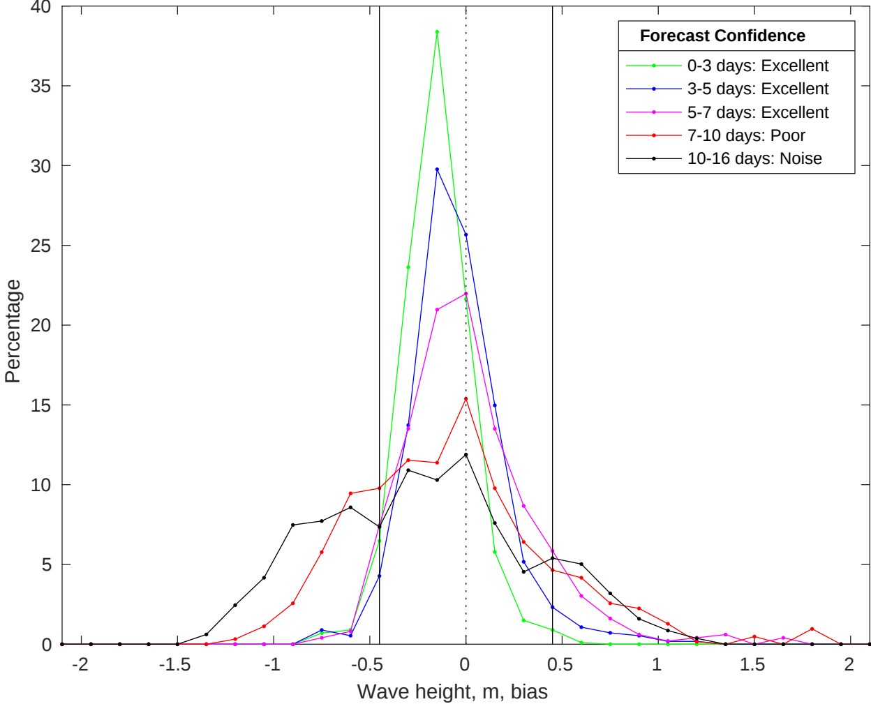
NDBC 46011 vs GFS Waves Bias Histogram: 14-Jul-2025
