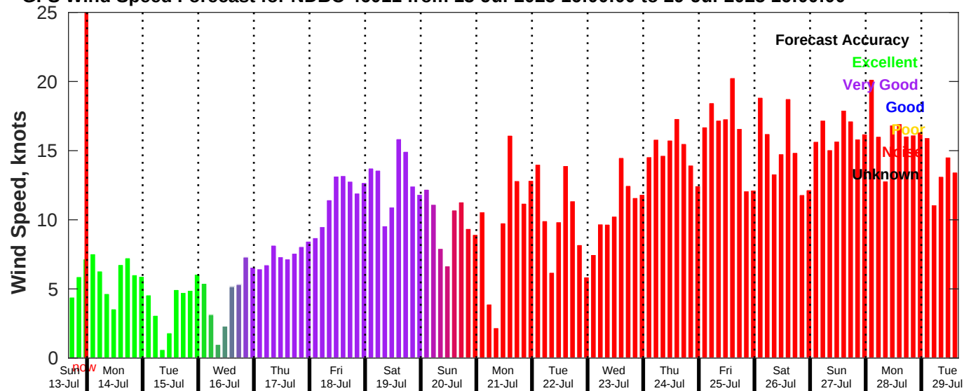
GFS Wind Speed Forecast for NDBC 46011 from 13-Jul-2025 16:00:00 to 29-Jul-2025 16:00:00
