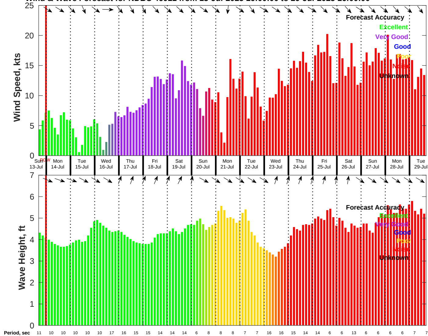
Wind & Wave Forecast for NDBC 46011 from 13-Jul-2025 16:00:00 to 29-Jul-2025 16:00:00
