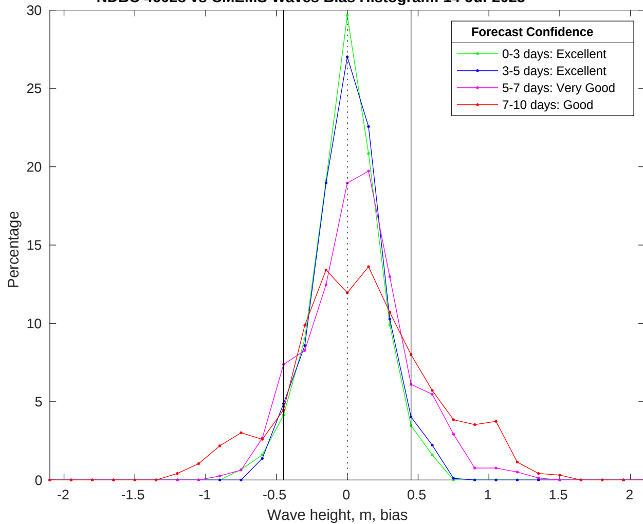
NDBC 46028 vs CMEMS Waves Bias Histogram: 14-Jul-2025
