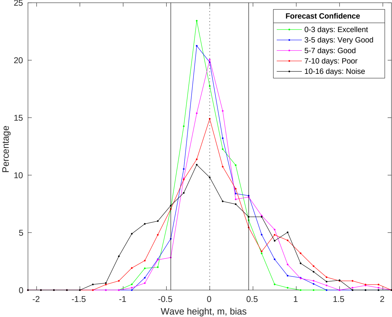
NDBC 46028 vs GFS Waves Bias Histogram: 14-Jul-2025
