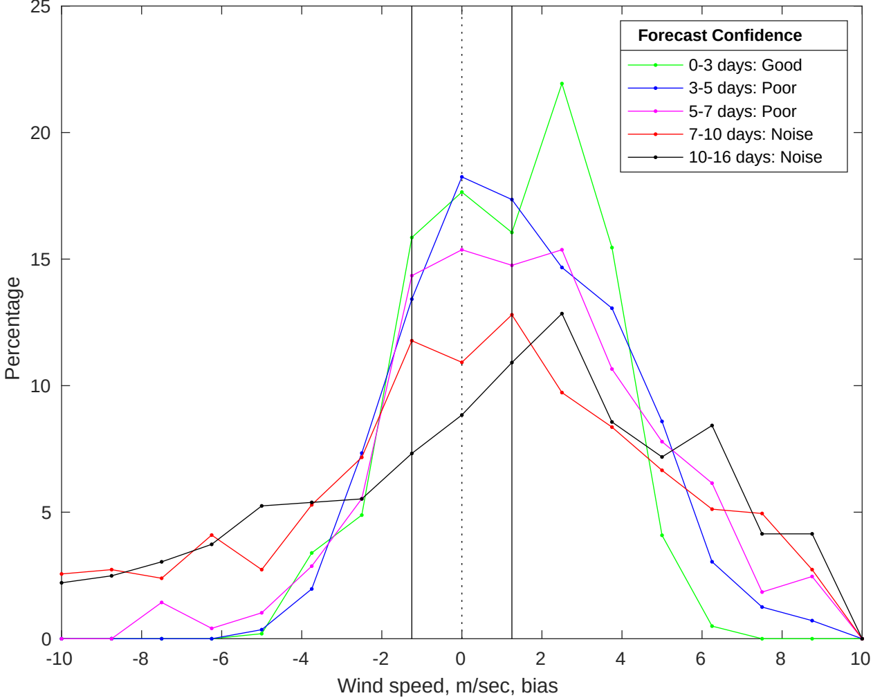
NDBC 46028 vs GFS Winds Bias Histogram: 14-Jul-2025
