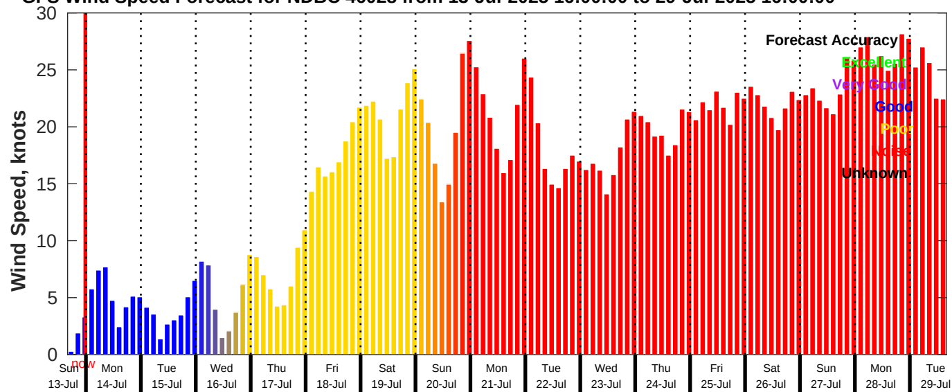
GFS Wind Speed Forecast for NDBC 46028 from 13-Jul-2025 16:00:00 to 29-Jul-2025 16:00:00
