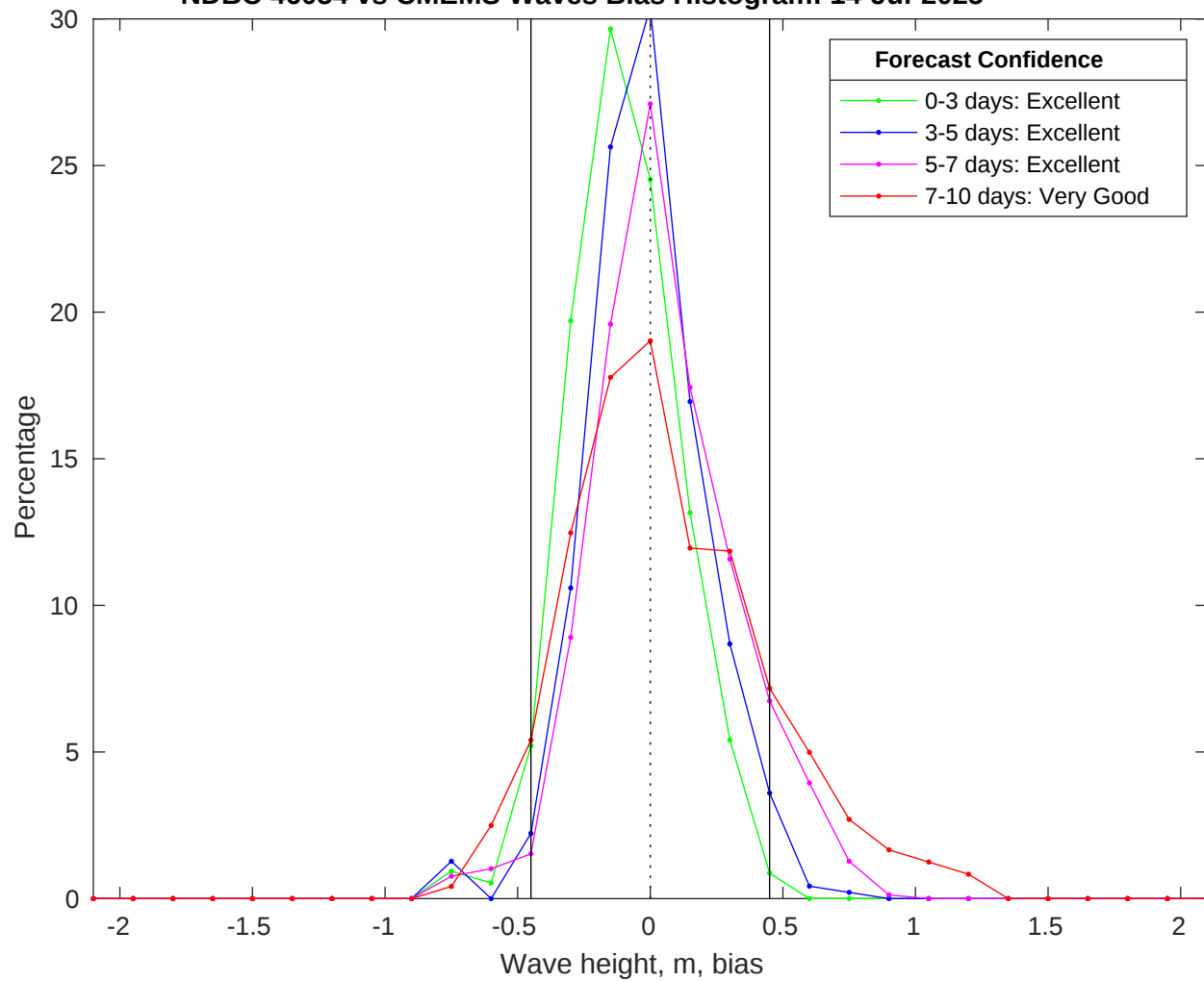
NDBC 46054 vs CMEMS Waves Bias Histogram: 14-Jul-2025
