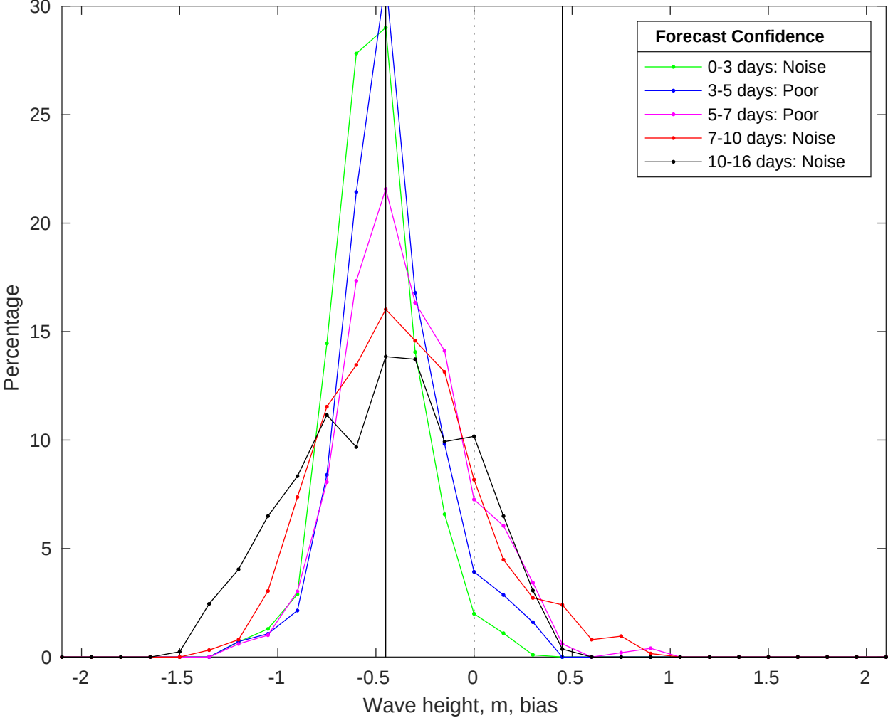
NDBC 46054 vs GFS Waves Bias Histogram: 14-Jul-2025
