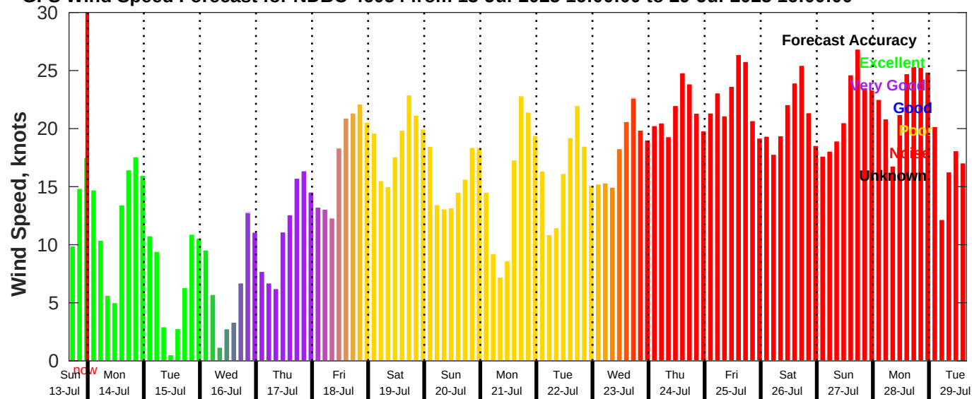
GFS Wind Speed Forecast for NDBC 46054 from 13-Jul-2025 16:00:00 to 29-Jul-2025 16:00:00
