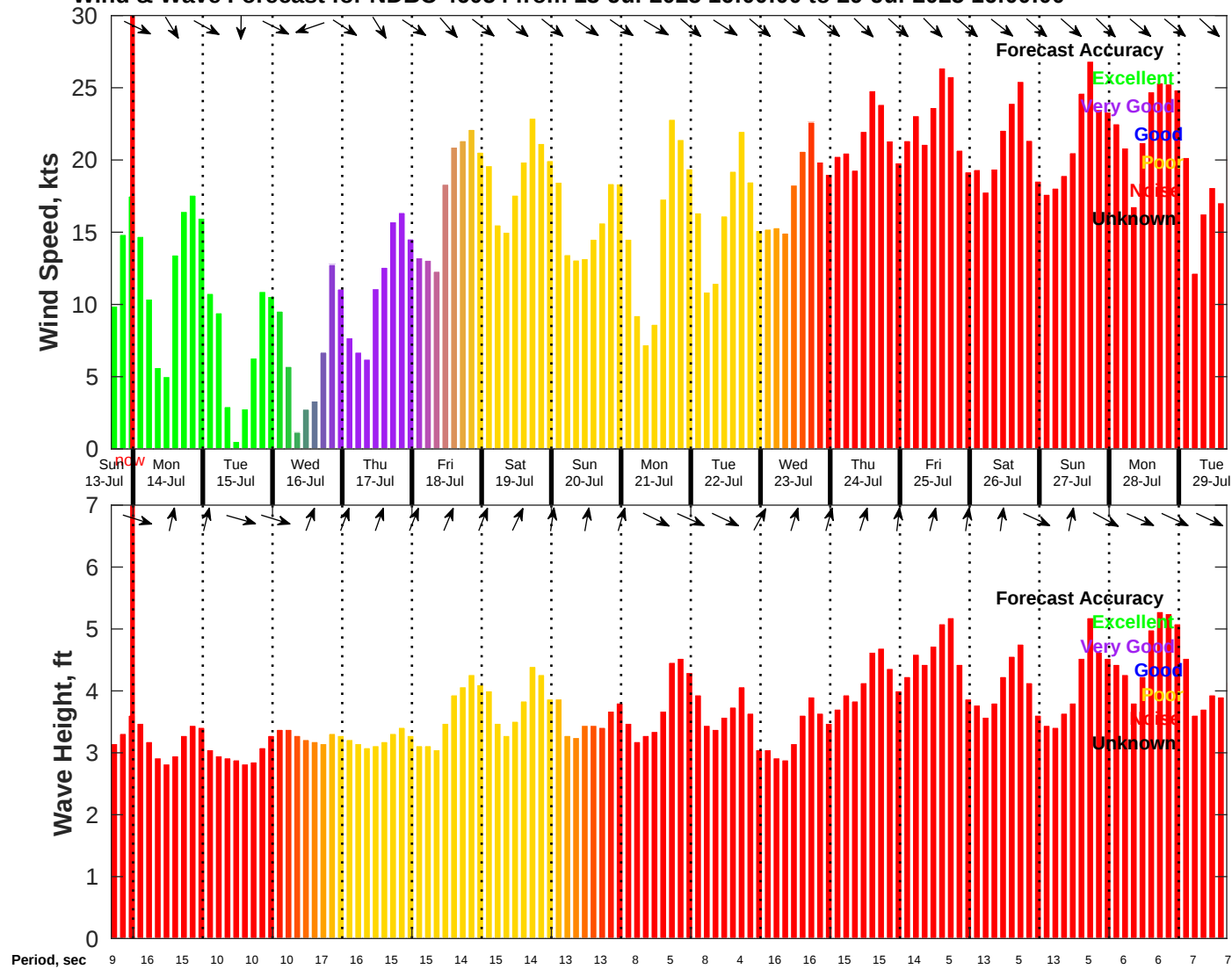
Wind & Wave Forecast for NDBC 46054 from 13-Jul-2025 16:00:00 to 29-Jul-2025 16:00:00
