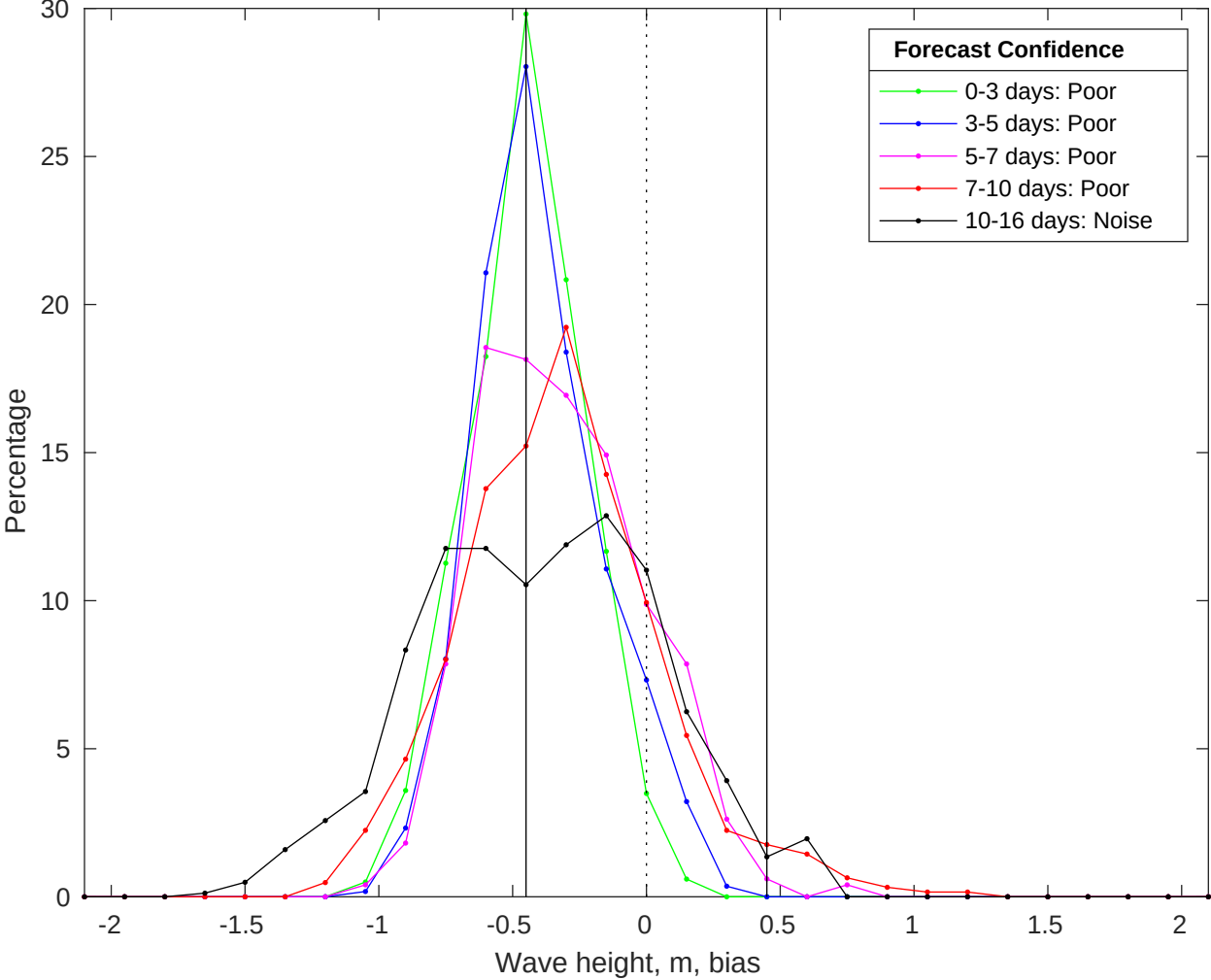
NDBC 46069 vs GFS Waves Bias Histogram: 14-Jul-2025
