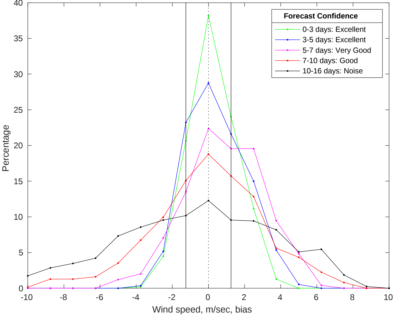
NDBC 46069 vs GFS Winds Bias Histogram: 14-Jul-2025
