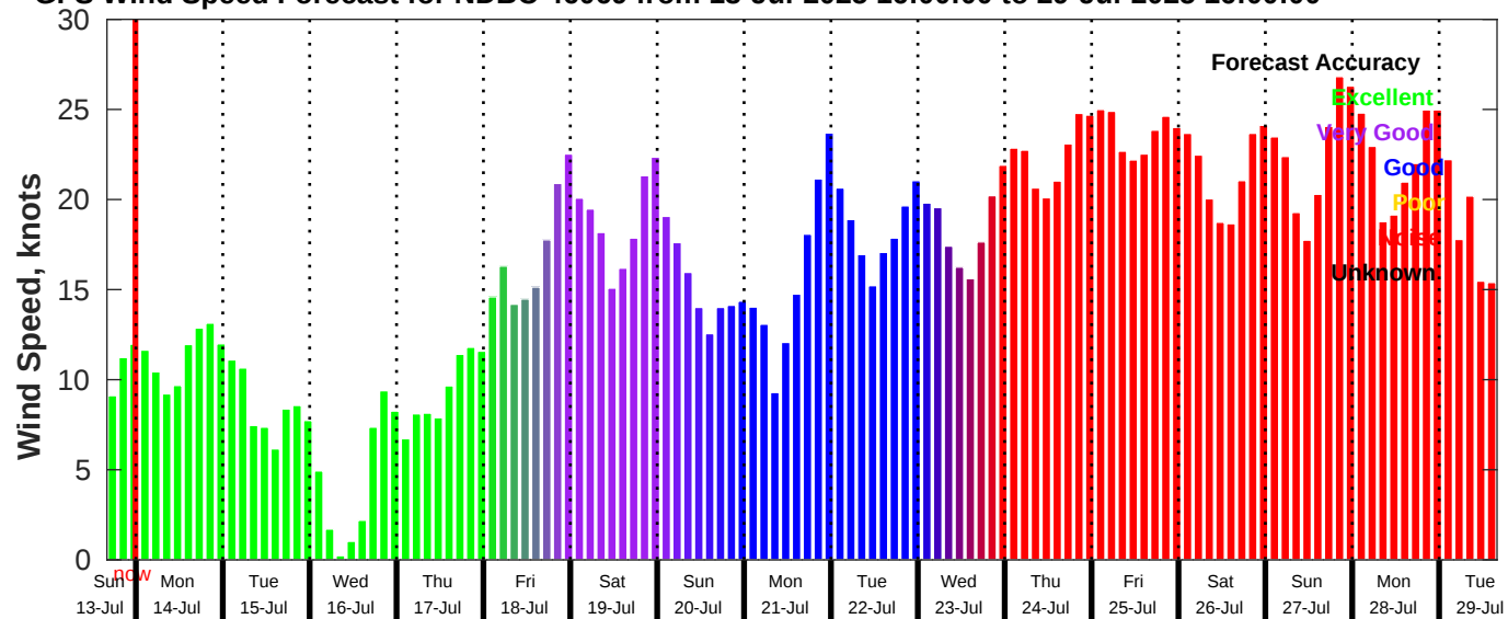
GFS Wind Speed Forecast for NDBC 46069 from 13-Jul-2025 16:00:00 to 29-Jul-2025 16:00:00
