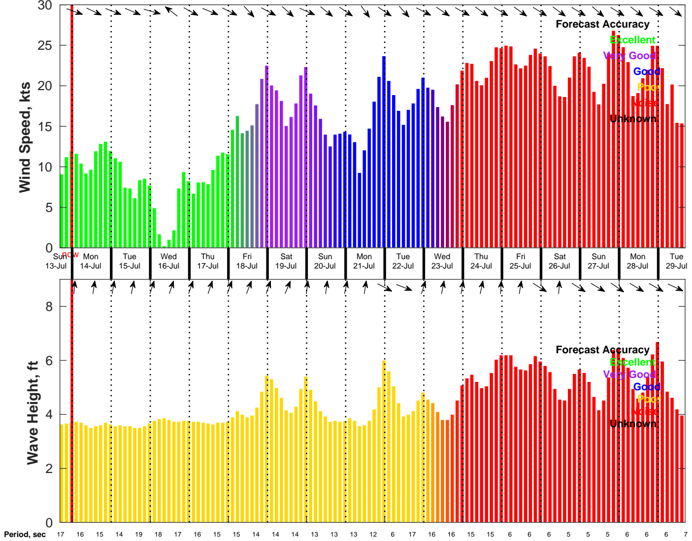
Wind & Wave Forecast for NDBC 46069 from 13-Jul-2025 16:00:00 to 29-Jul-2025 16:00:00
