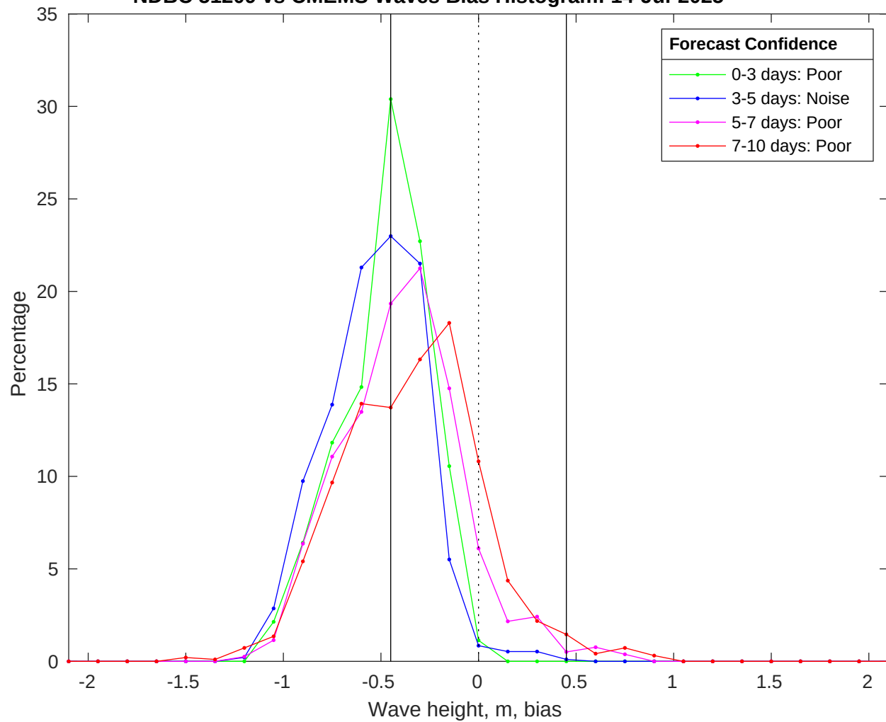
NDBC 51209 vs CMEMS Waves Bias Histogram: 14-Jul-2025
