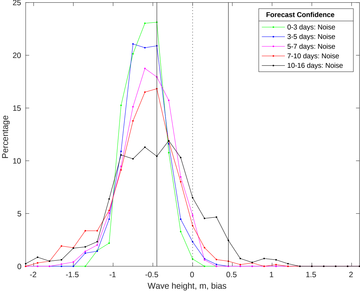
NDBC 51209 vs GFS Waves Bias Histogram: 14-Jul-2025
