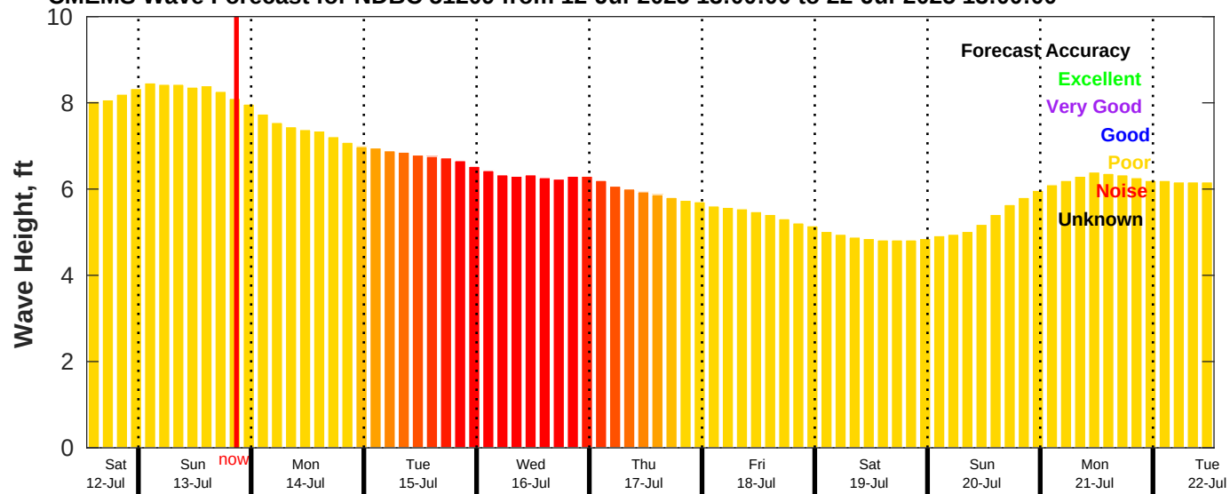
CMEMS Wave Forecast for NDBC 51209 from 12-Jul-2025 13:00:00 to 22-Jul-2025 13:00:00
