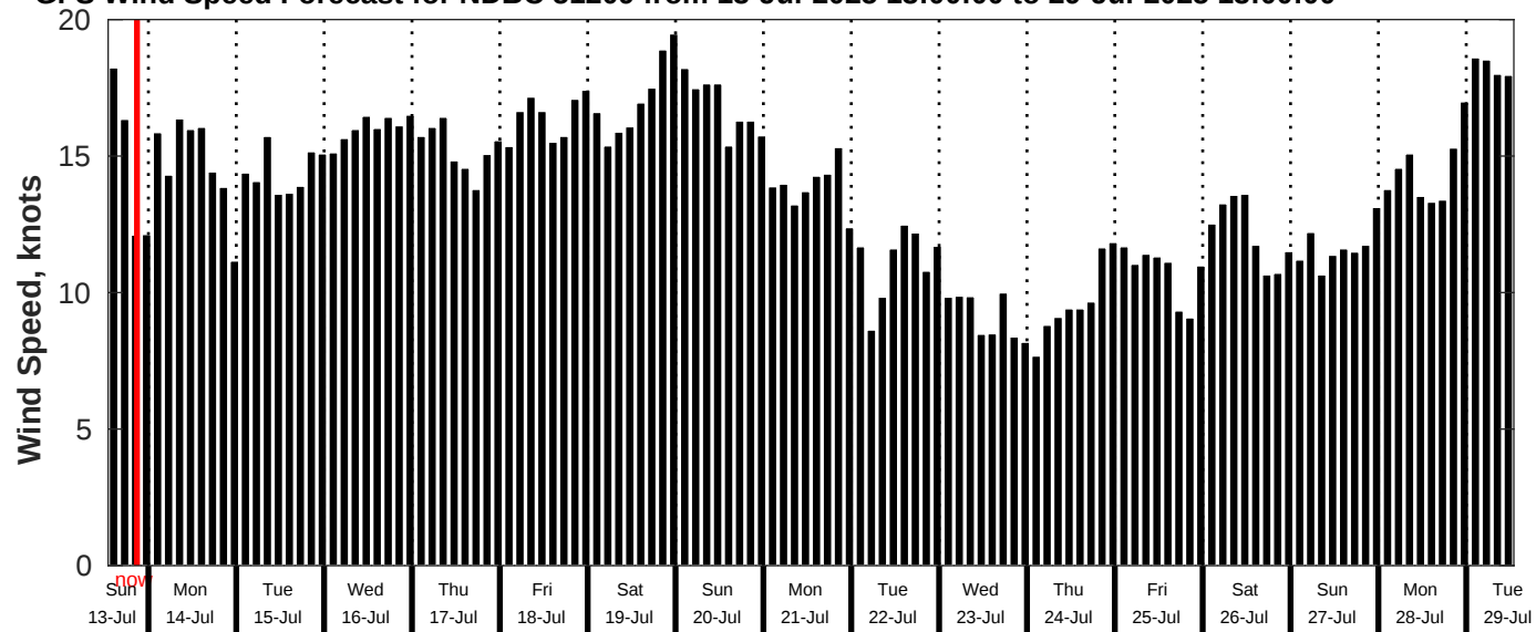
GFS Wind Speed Forecast for NDBC 51209 from 13-Jul-2025 13:00:00 to 29-Jul-2025 13:00:00
