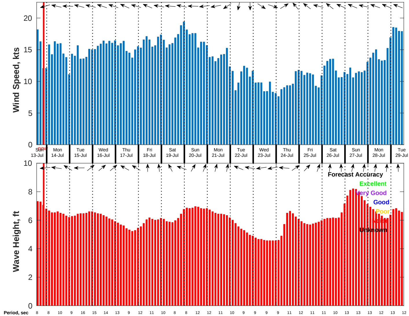
Wind & Wave Forecast for NDBC 51209 from 13-Jul-2025 13:00:00 to 29-Jul-2025 13:00:00
